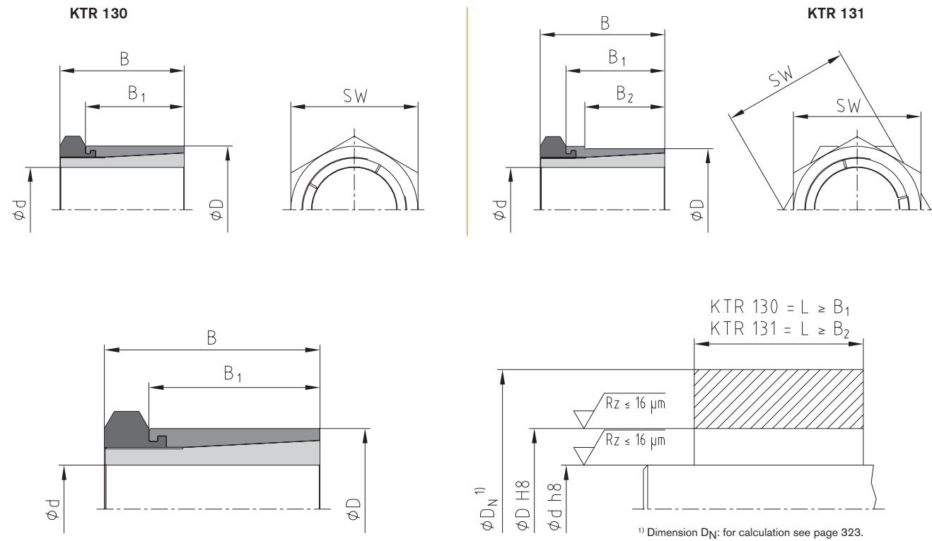
Example of application of hub type
